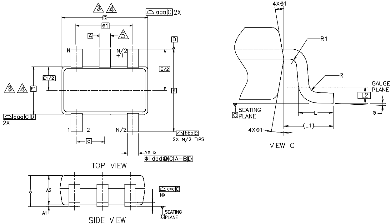
Figure 21. TSOT23-5 Package
